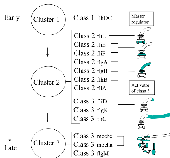
Fig. 3. Present kinetic classification of the flagellar operons. The three clusters and the operons within each cluster are arranged by their relative timing according to the temporal clustering results. Positions of the corresponding gene products in the flagellum (1) are indicated in green.
